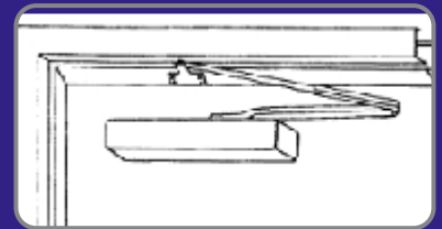
Parallel Arm(Push Side) Permit 180° maximum opening
